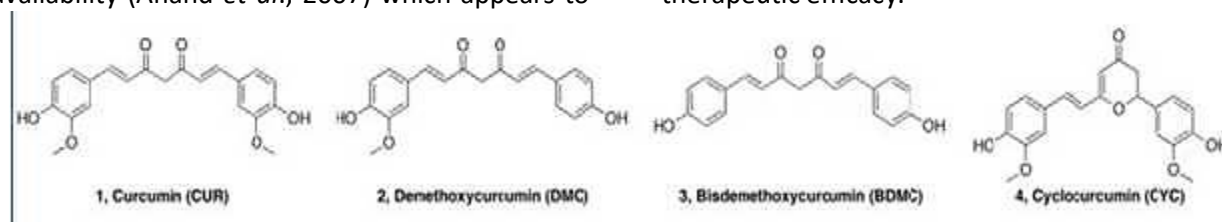
Chemical Structure of curcuminoids
